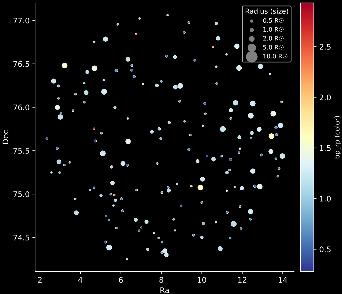
APOGEE DR17 Field: [CVZTILE_107+30_btx] Stars: 166
