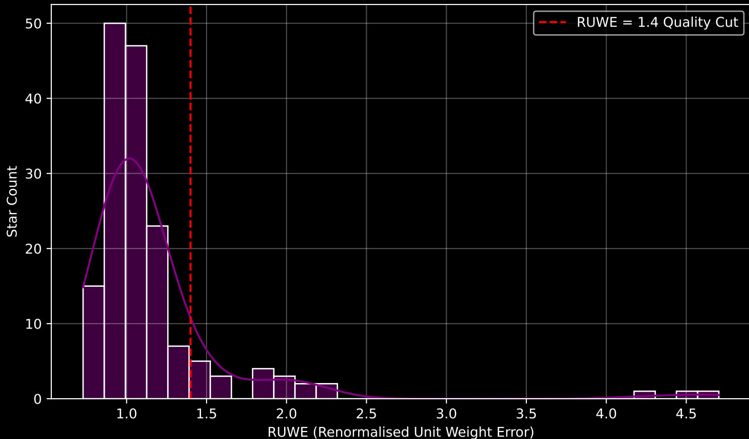
GAPOGEE DR17 Field [CVZTILE_107+30_btx] RUWE Distribution (n= 164)
