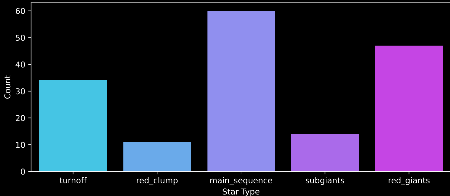
APOGEE DR17 Field: [CVZTILE_107+30_btx] Count plot of Star Type
