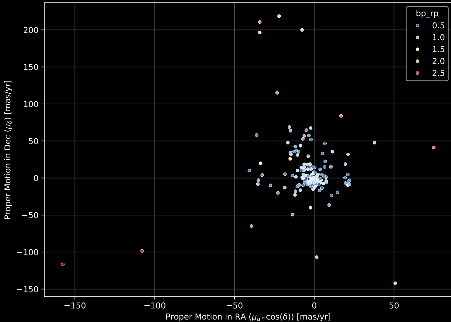
APOGEE DR17 Field: [CVZTILE_107+30_btx] Proper Motion Diagram (n= 166)
