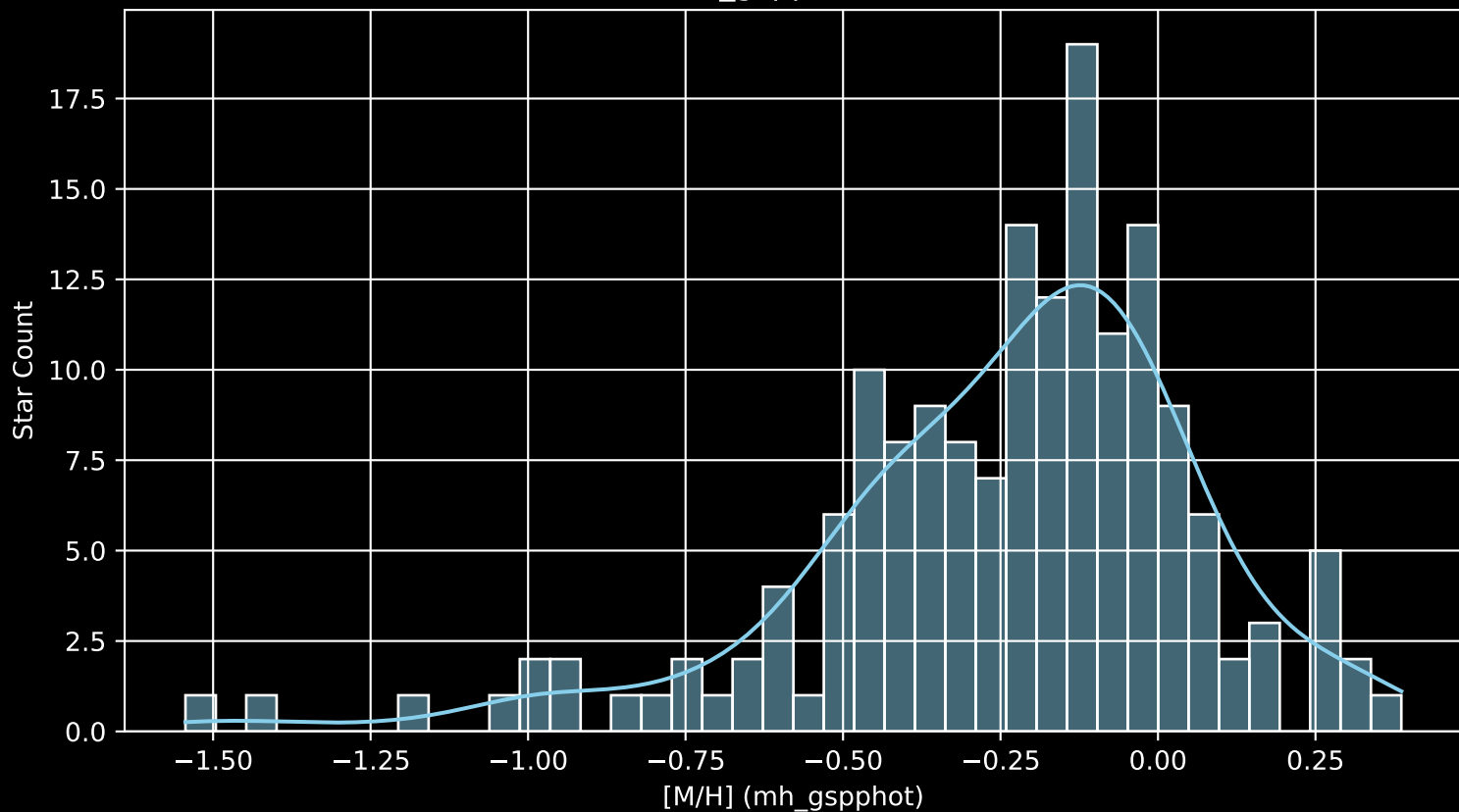
APOGEE DR17 Field: [CVZTILE_107+30_btx [M/H] (mh_gspphot) (n= 166)
