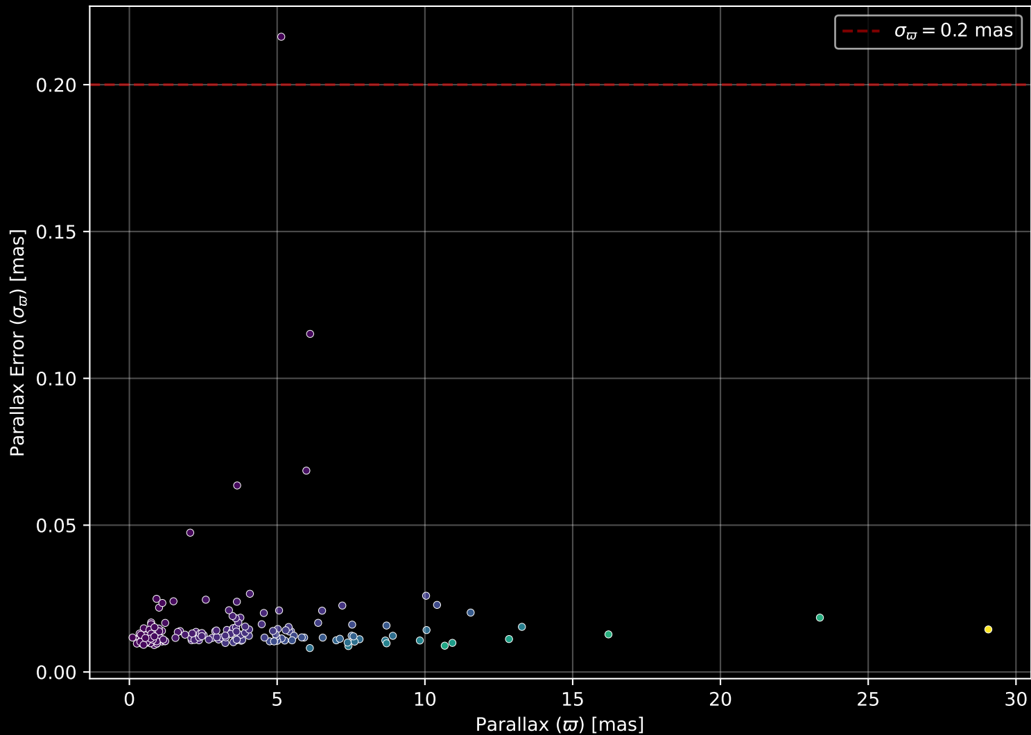
APOGEE DR17 Field: [CVZTILE_107+30_btx] Parallax Quality (n= 166)
